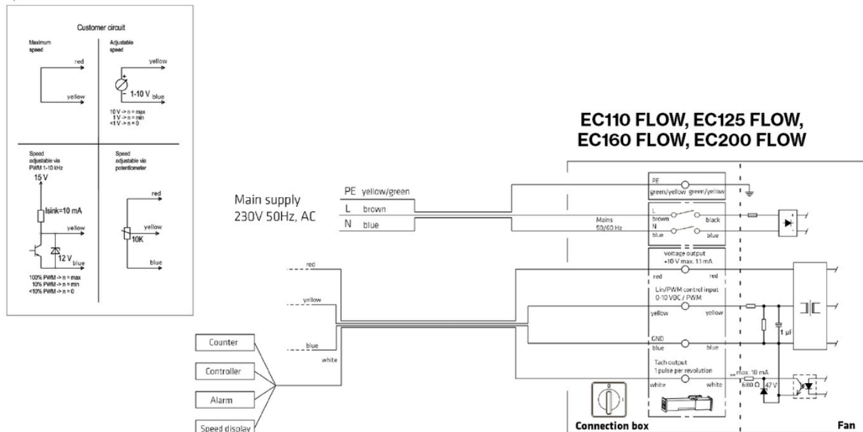
Speed Controller
