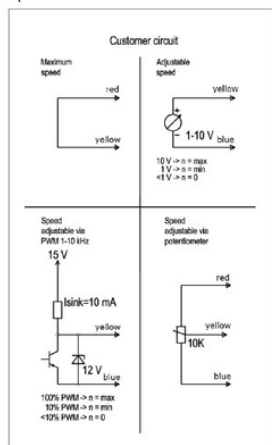
Speed Controller
