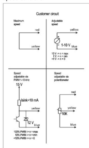
Speed Controller
