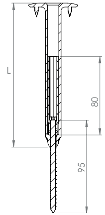
VILPE Croco A fastener + Adjustable Croco screw 95. L is the length of the Croco model.
