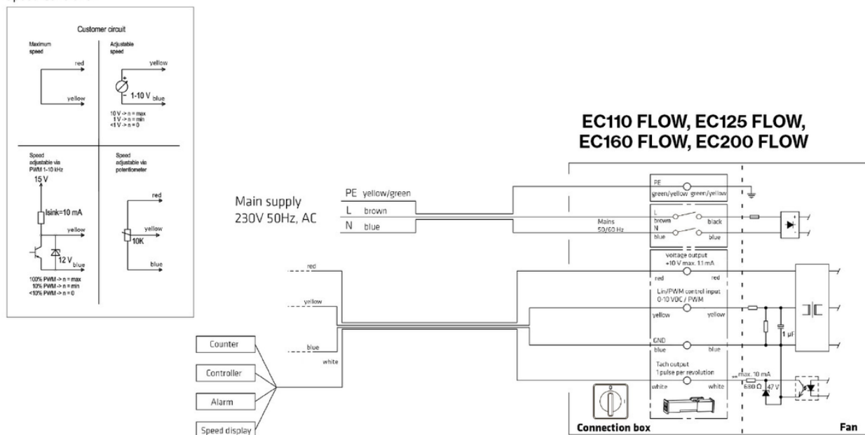
Speed Controller
