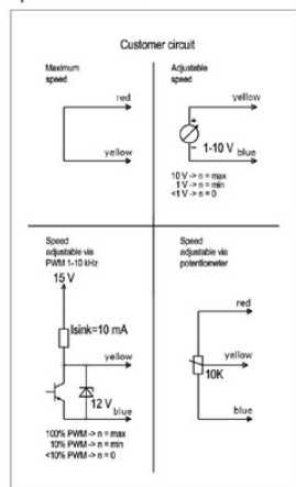
Speed Controller
